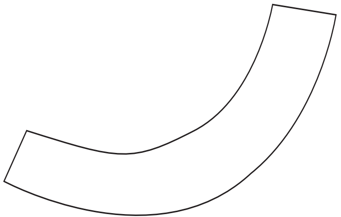
Spaceship Pattern
