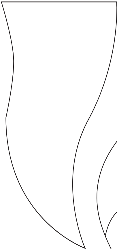
Pennant Pattern
