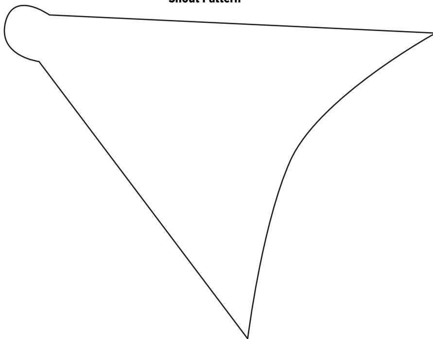
Snout Pattern
